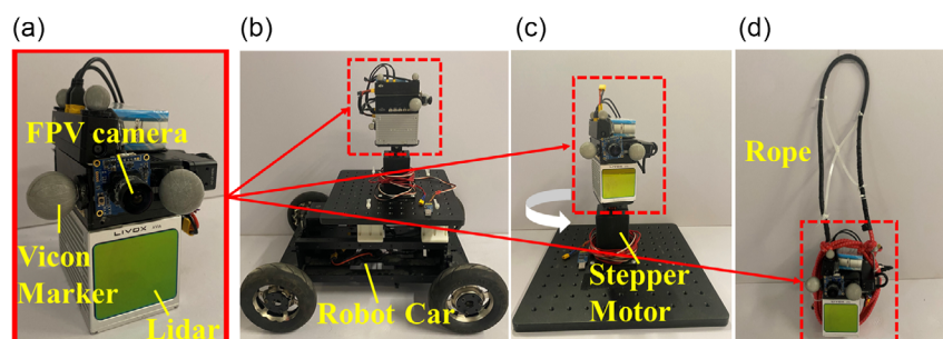
Figure 3. Experimental platforms for evaluations. a) The sensor suite consisting of a Livox Avia LiDAR, a FPV camera, and five Vicor Markers. The sensor suite is carried by b) a robot car, c) a rotating platform driven by a step motor, and d) a pendulum.
