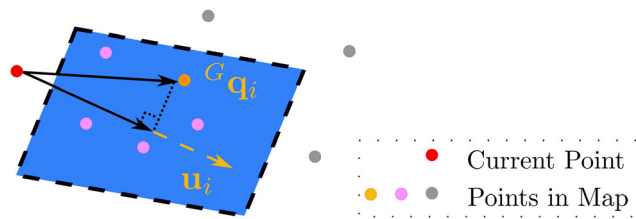
Figure 2. Illustration of direct registration of LiDAR point to map. {}^G\mathbf{q}_i and \mathbf{u}_i refer to a point in the map and the normal vector of the plane in blue.
